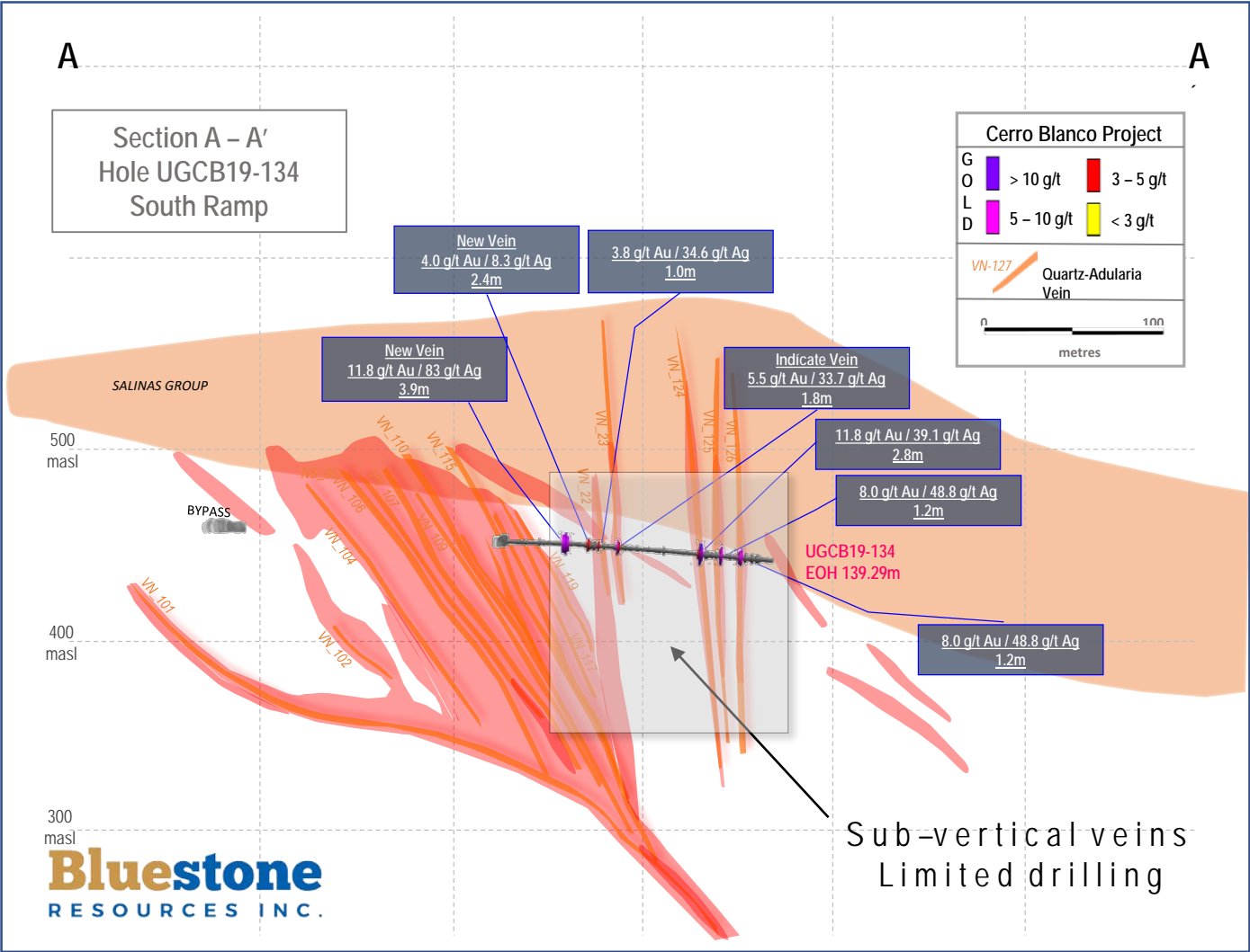
Figure 2 Section A – A'
